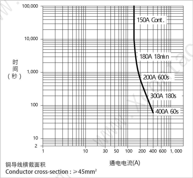
过载电流参考曲线-图2 Overload Current vs Time Reference Curve-Graph2
