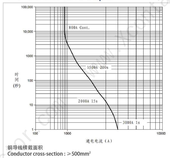
过载电流参考曲线-图2 Overload Current vs Time Reference Curve-Graph2
