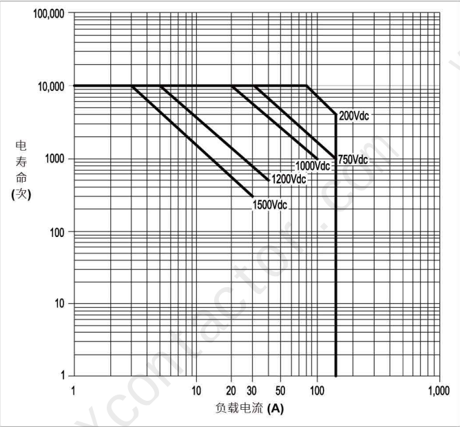
电气寿命参考曲线-图1 Electrical Life Reference Curve-Graph1
