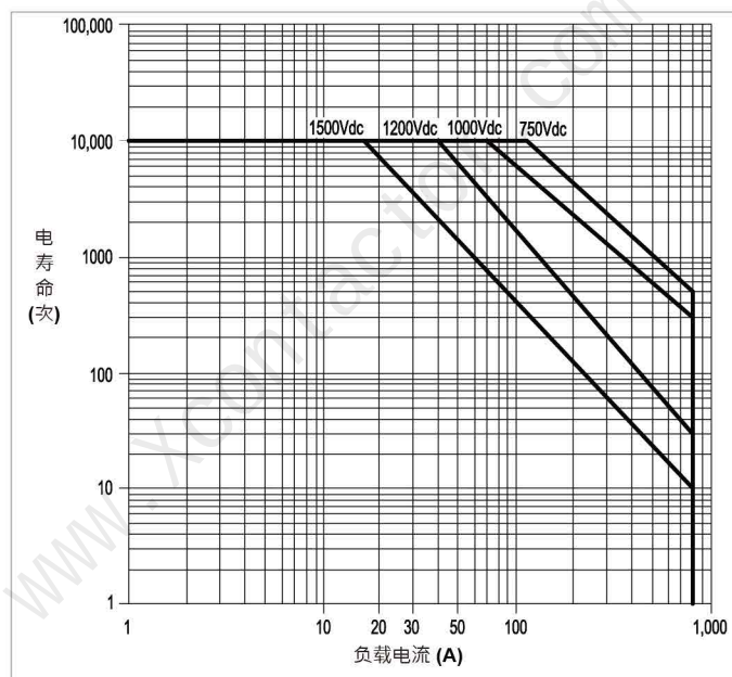
电气寿命参考曲线-图1 Electrical Life Reference Curve-Graph1
