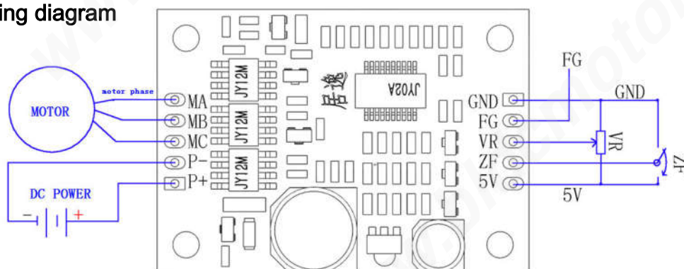
Driver board diagram
