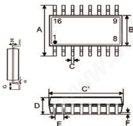
SOP16 packaging
