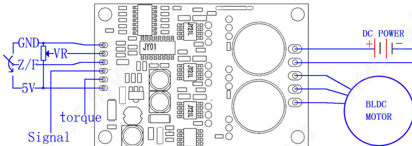
Wiring diagram
