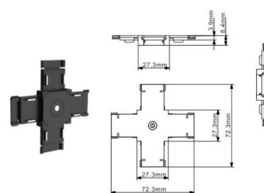
Four direction module
