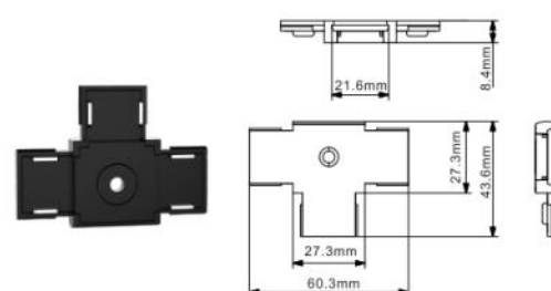
Three direction module
