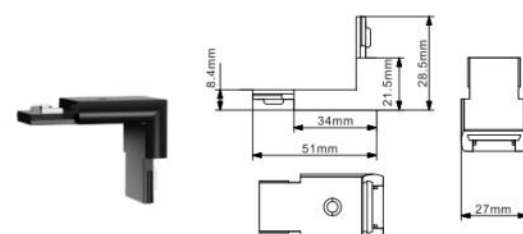
IN corner module
