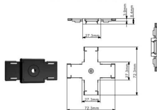
Pass-through module
