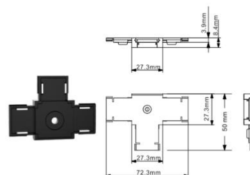
Three direction module
