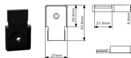
Rail plug fixing parts
