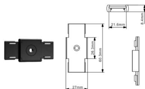
Pass-through module
