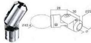
Crossbar holder, tube-bar 穿棒件, 管-棒 MODEL: SJ-H184 Φ: 8-12
