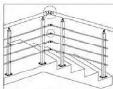
End cap, thread-arched 封头, 螺牙-弧形 MODEL: SJ-H151 Φ: 38/42.4/48.3/50.8
