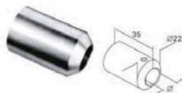
Crossbar holder, flat-bar 穿棒件, 平-棒 MODEL: SJ-H179 Φ: 8-12
