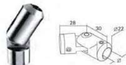
Crossbar holder, flat-bar 穿棒件, 平-棒 MODEL: SJ-H181 Φ: 8-12
