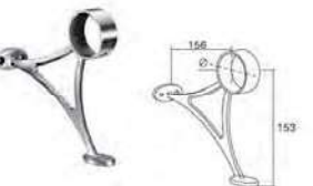
Handrail bracket 扶手托架 MODEL: SJ-H129 Φ: 42.4/50.8
