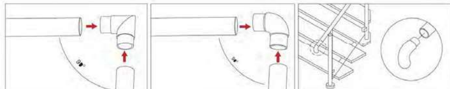
Elbow, adjustable 弯头, 可调节 MODEL: SJ-H139 Φ: 42.4/50.8
