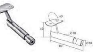
Handrail bracket 扶手托架 MODEL: SJ-H128 Φ: 42.4/50.8
