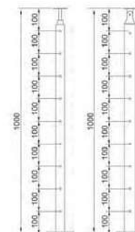
Cable tensioner 钢丝绳紧固件 MODEL: SJ-H070 Φ: 5-8
