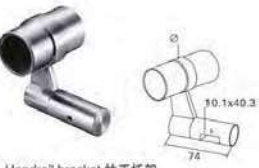
Handrail bracket 扶手托架 MODEL: SJ-H125 Φ: 42.4/50.8
